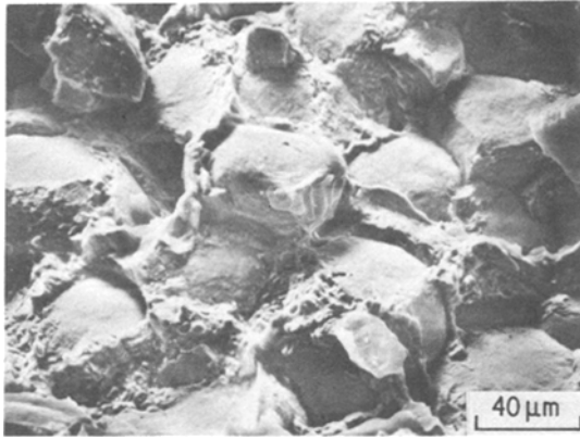
Figure 6 Appearance of tensile fracture region with tearing of interparticle melt regions.
