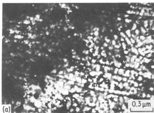
Figure 12 Gamma prime precipitates formed after ageing at (a) 950° C/1 h and (b) 1150° C/1 h observed by transmission electron microscopy.
