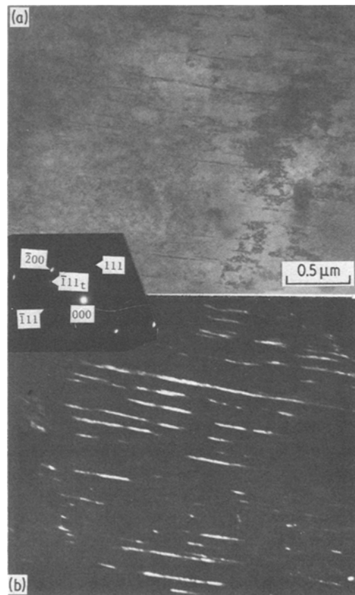
Figure 9 Substructure exhibiting deformation twins after ageing consolidated alloy for one hour at 600 °C; (a) bright field, (b) dark field of \bar{1}11_t reflection showing twins.
