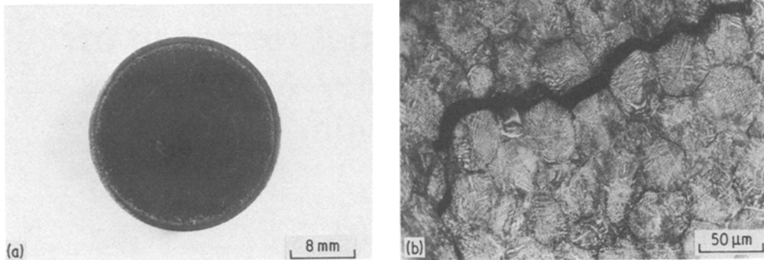
Figure 1 Cracks developed during consolidation using axi-symmetric system. (a) Radial and circumferential cracks. (b) Micrograph showing how cracks propagate in an interparticle mode.
